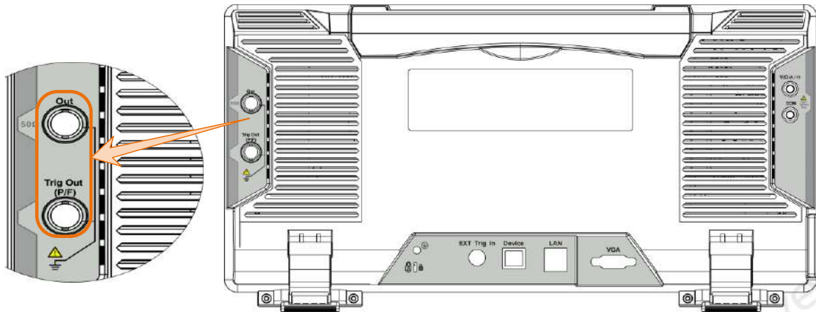
Figure 4-1 Generator Output Ports (Dual-channel)
