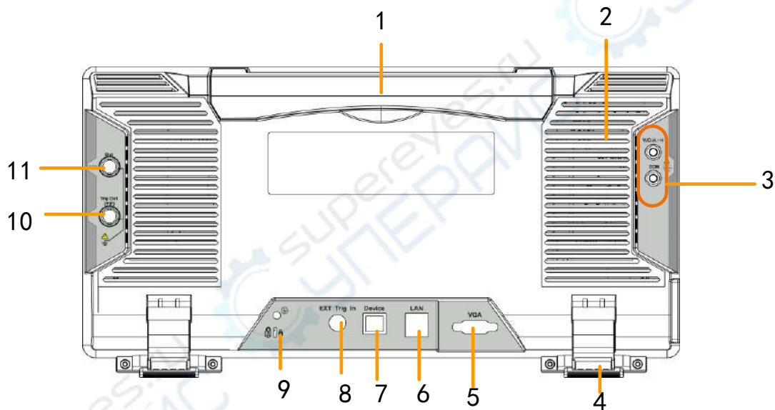
Figure 3-2 Rear Panel
