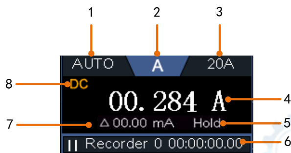
Figure 5-3 Multimeter Information Window
