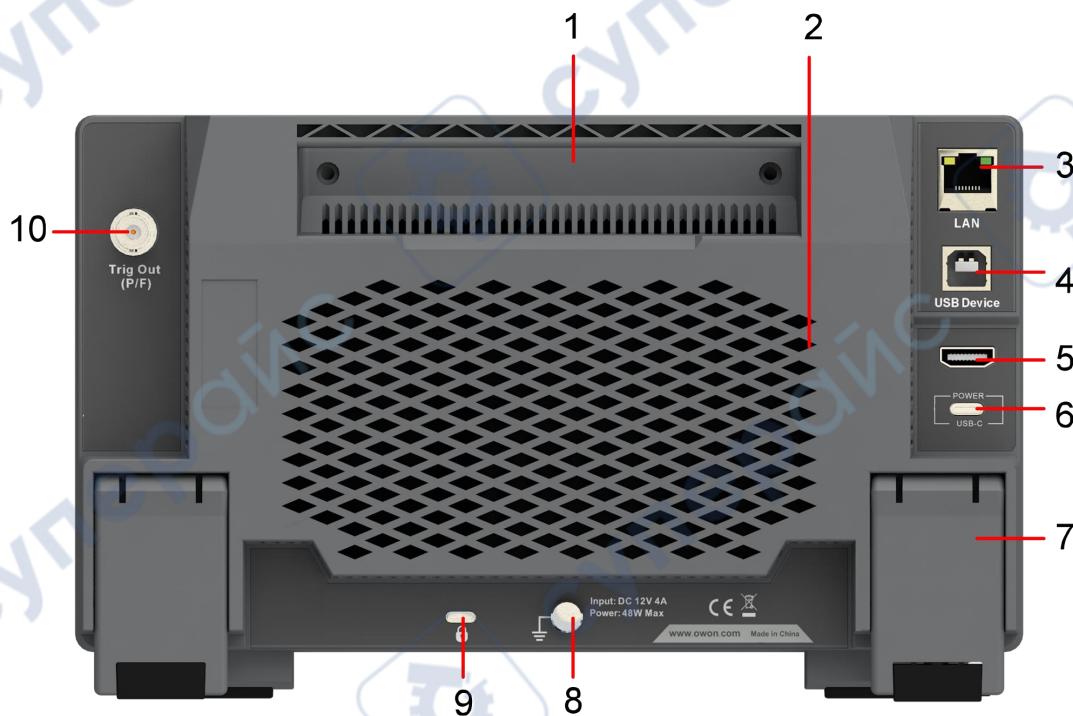
Figure 3-2: Rear Panel
