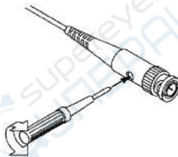
Figure 0-3: Probe Adjustment
