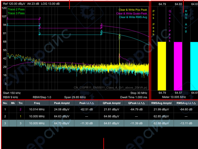
Signal list and its final measurement results are displayed Figure 6-1 EMI measurement interface
