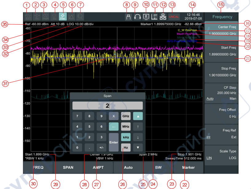
Figure 4-4 User interface
