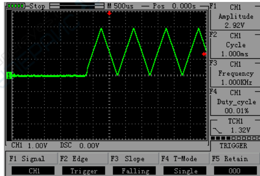
Figure 2-16 single trigger
