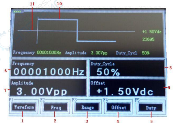
Figure 3-1 signal generator interface
