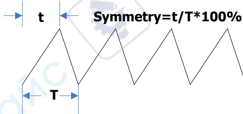
Figure 17-1 Symmetry Definition
