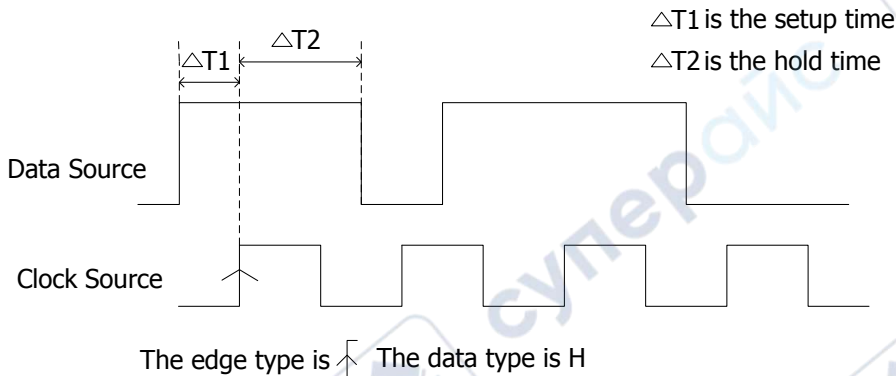
Figure 5-11 Setup/Hold Trigger
