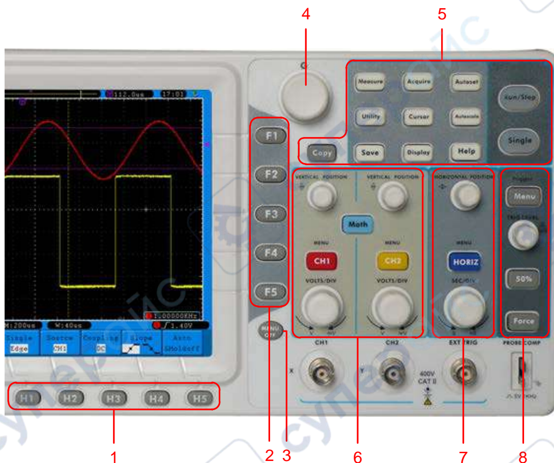
Figure 4-4 Keys Overview
