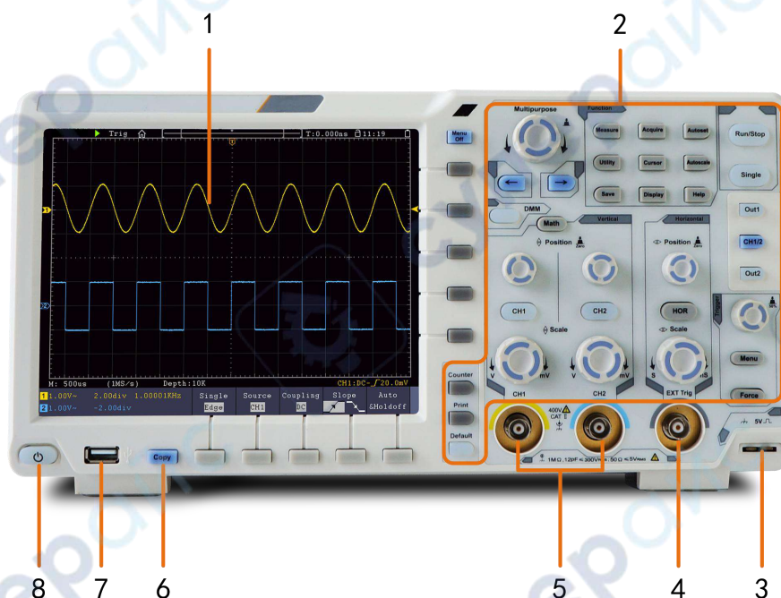
Figure 3- 1 Front panel
