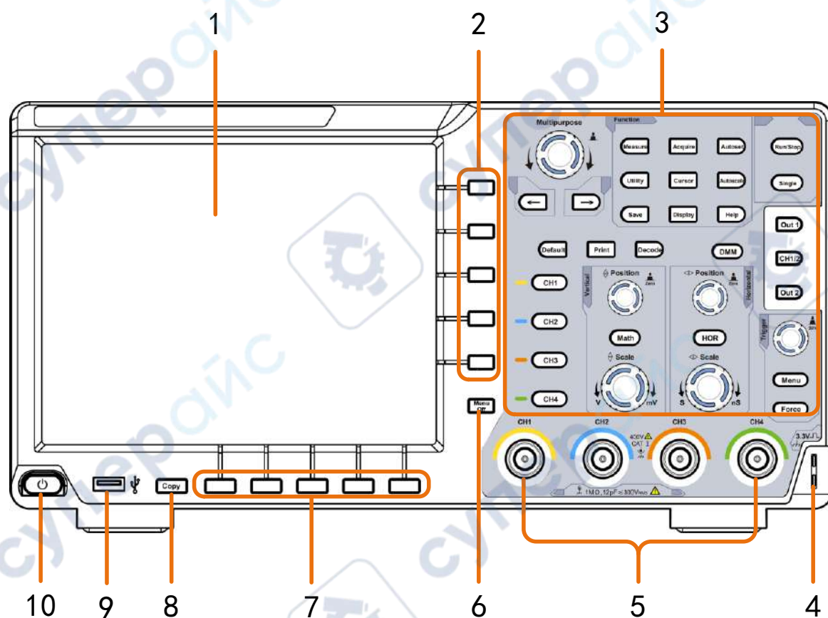
Figure 3-1 Front panel
