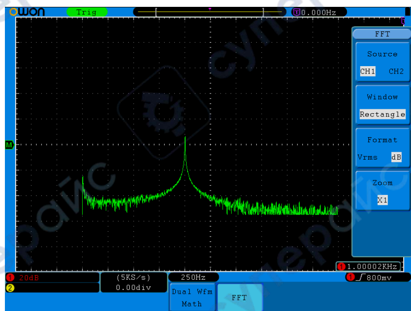
Figure 5-11 Rectangle window
