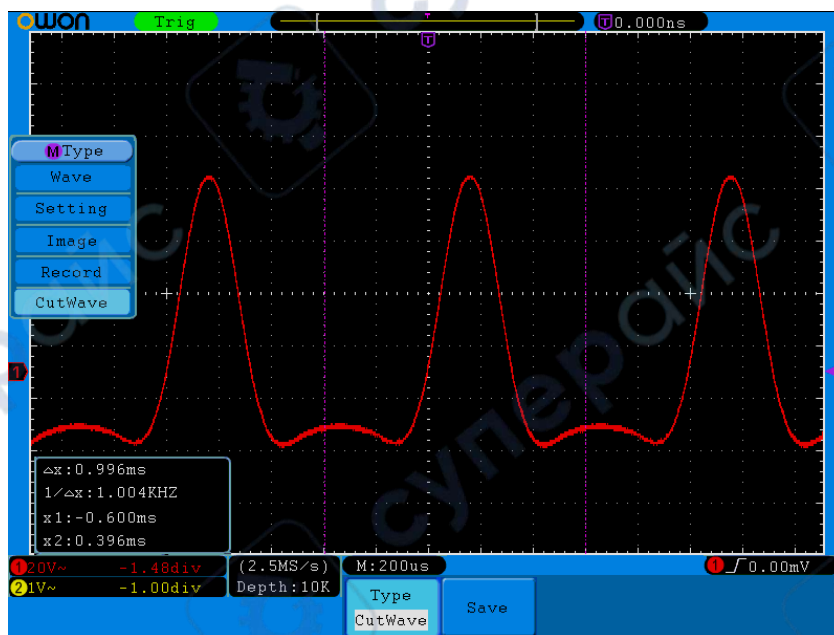
Figure 5-49: Cut Wave
