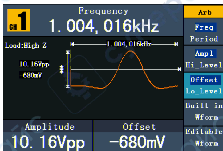
Figure 5-52: Read file
