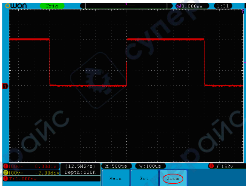
Figure 5-18 Zoom Window
