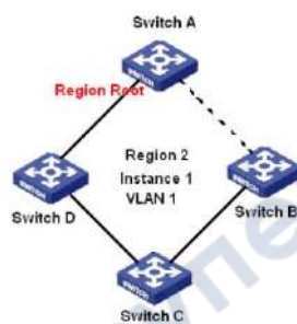
Рис. 159. Mapping to Instance 1
