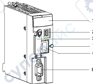
BMX P34 2030 Processor
