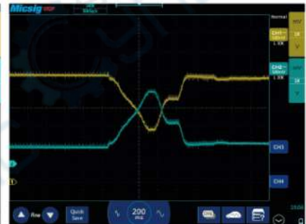
Throttle Position
