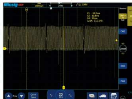
Crankshaft
