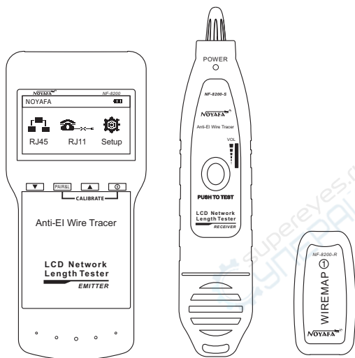
Main tester (NF-8200)
