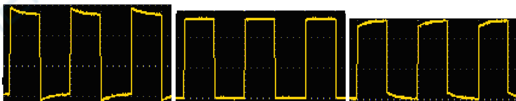
Figure 3-6 Displayed Waveforms of the Probe Compensation
