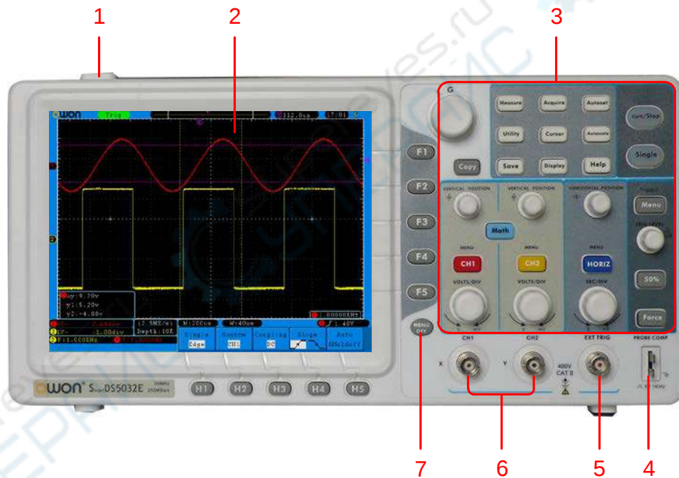
Figure 4-1 Front panel
