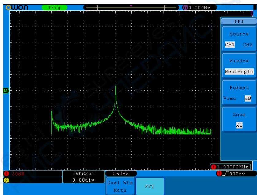
Figure 5-10 Rectangle window
