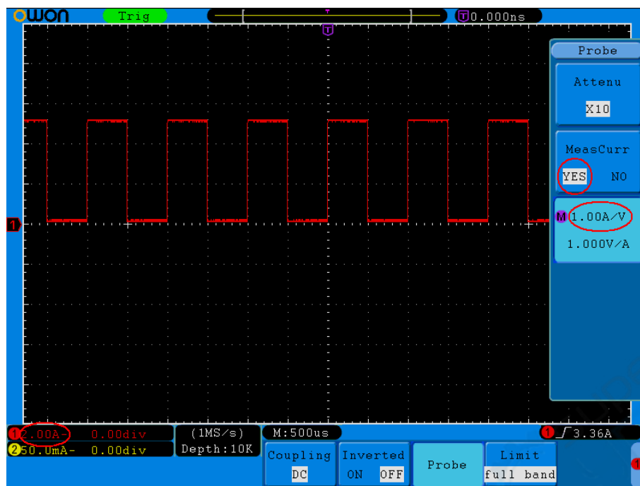
Figure 5-4 Measure Current
