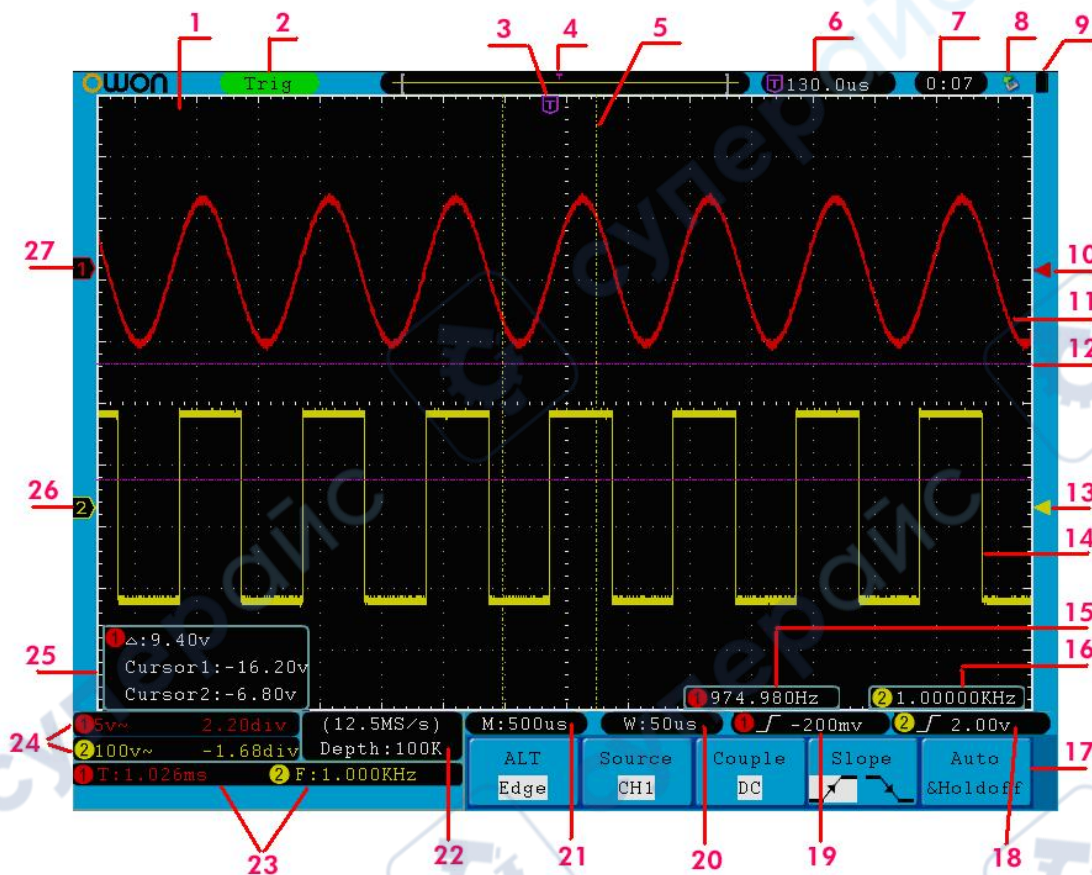
Fig. 4-6 Illustrative Drawing of Display Interfaces
