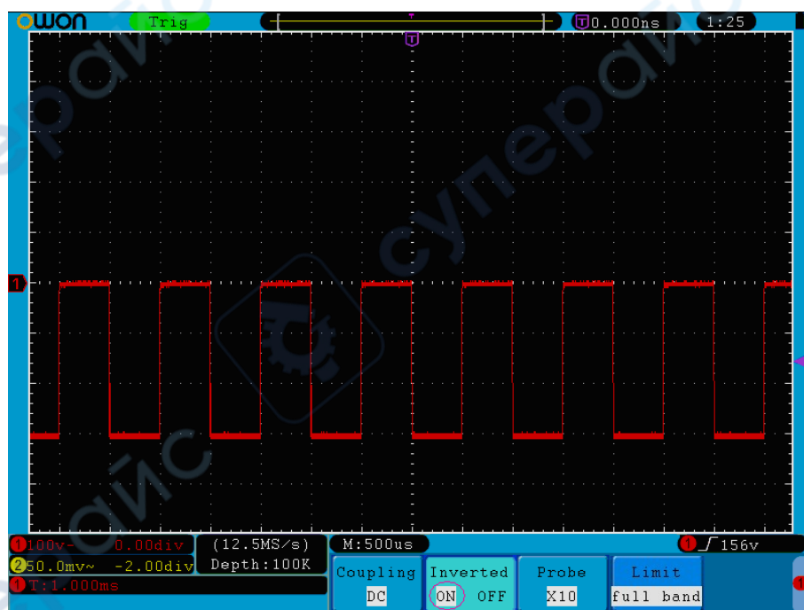
Fig. 5-5 Waveform Inverted
