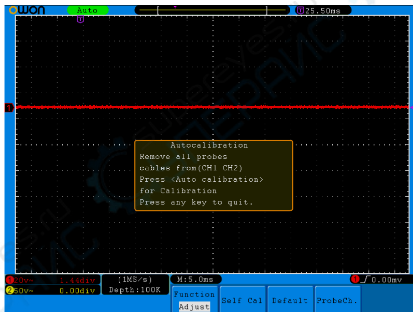
Figure 5-59 Self-Calibration
