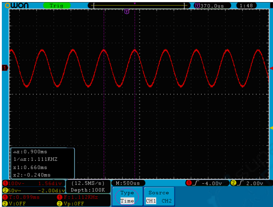
Figure 5-72 Waveform of Cursor Measurement
