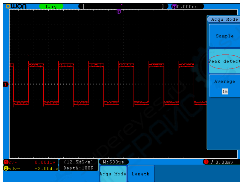
Figure 5-25 Peak Detect mode, under which the burrs on the falling edge of the square wave, can be detected and the noise is heavy.
