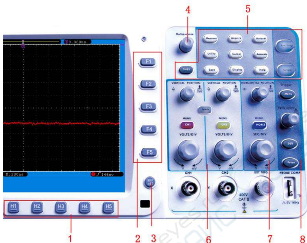
Figure 4-5 Keys Overview
