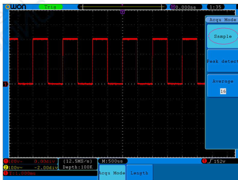
Figure 5-26 Normal ACQU Mode display, in which no burr can be detected.
