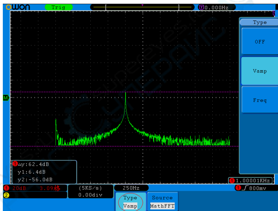
Figure 5-74 wave of Vamp cursor measurement
