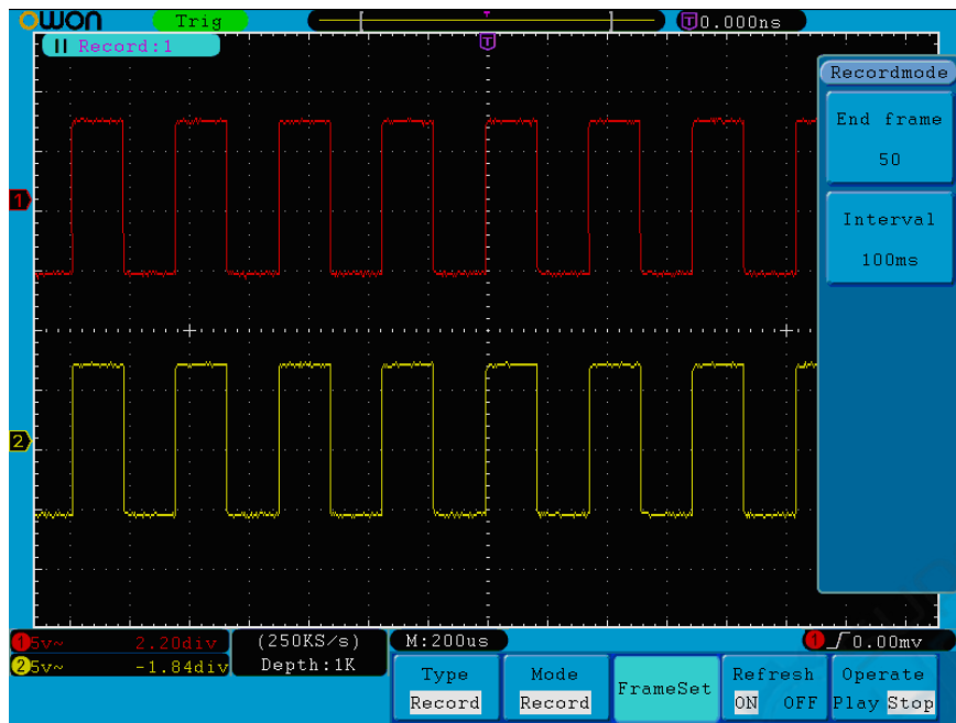
Figure 5-50 Wave Record
