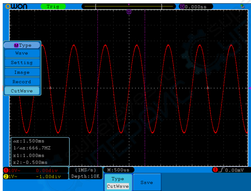
Figure 5-46: Cut Wave
