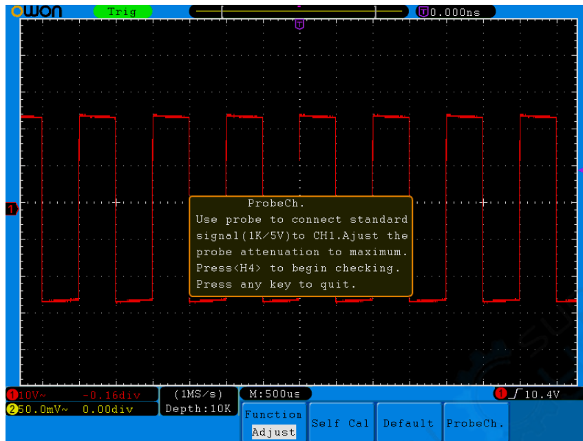
Figure 5-60: Probe Checking
