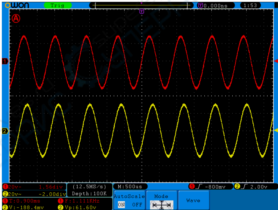
Figure 5-77 Autoscale Horizontal-Vertical multi-period waveforms
