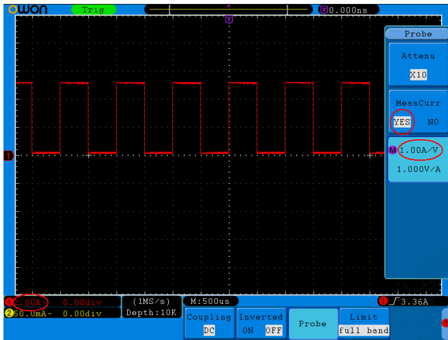
Figure 5-5 Measure Current
