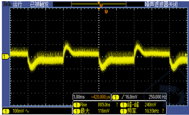
Figure 4, 25% - 50% load dynamic
