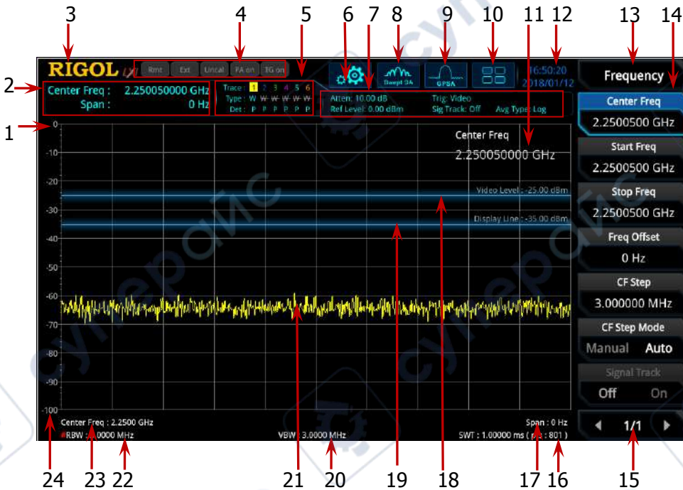
Figure 1-9 User Interface
