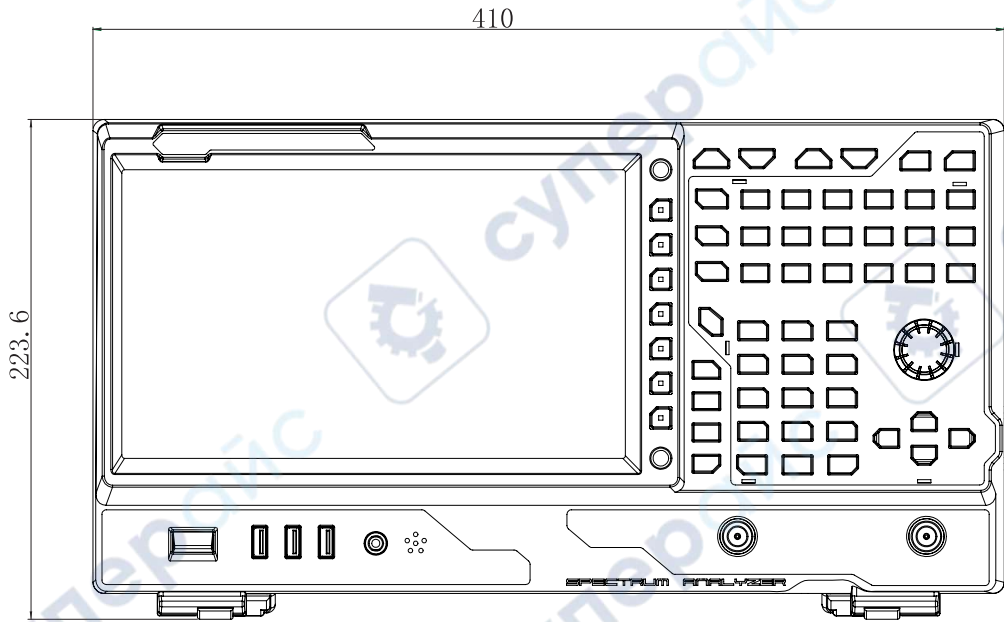
Figure 1-1 Front View
