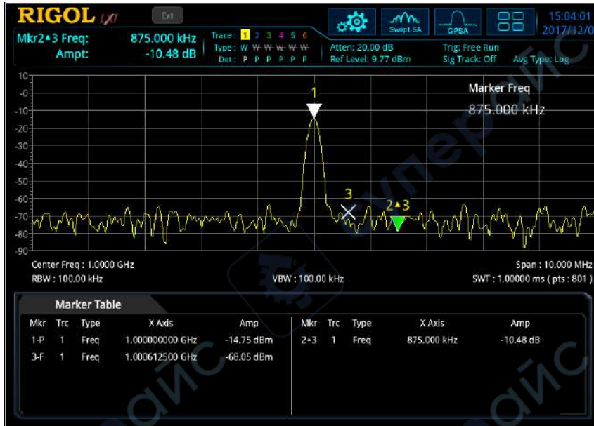
Figure 2-15 Marker Table
