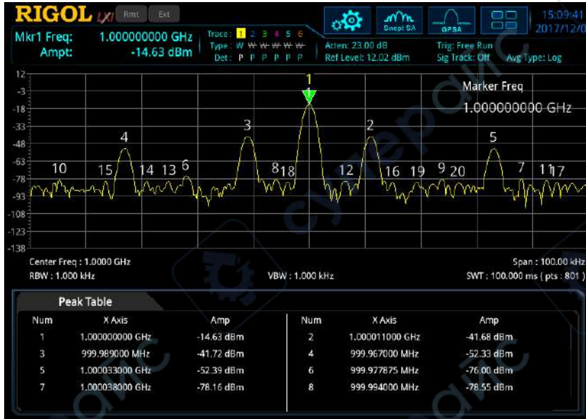
Figure 2-17 Peak Table
