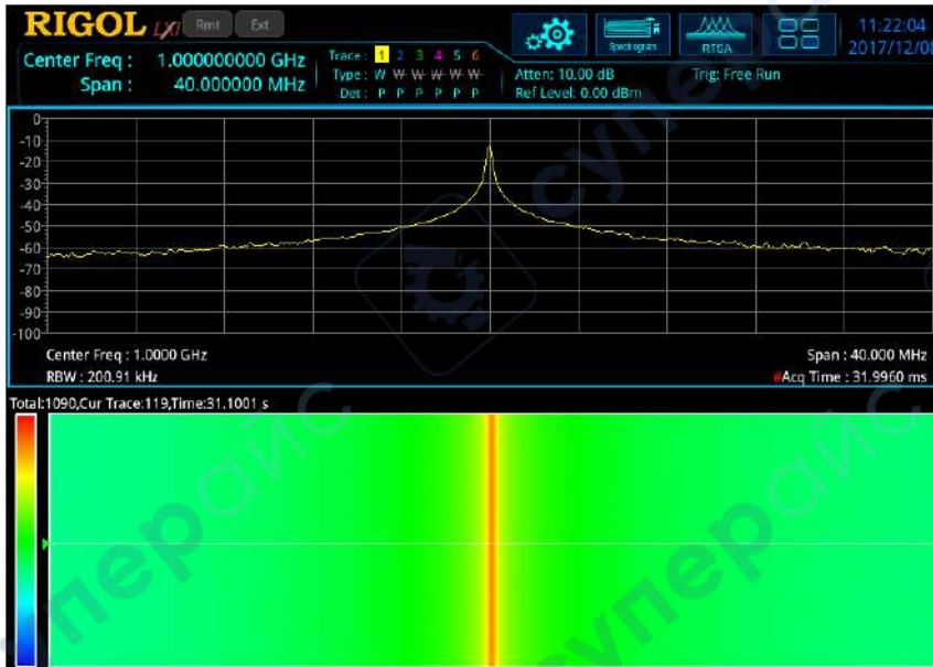
Figure 3-3 Spectrogram View
