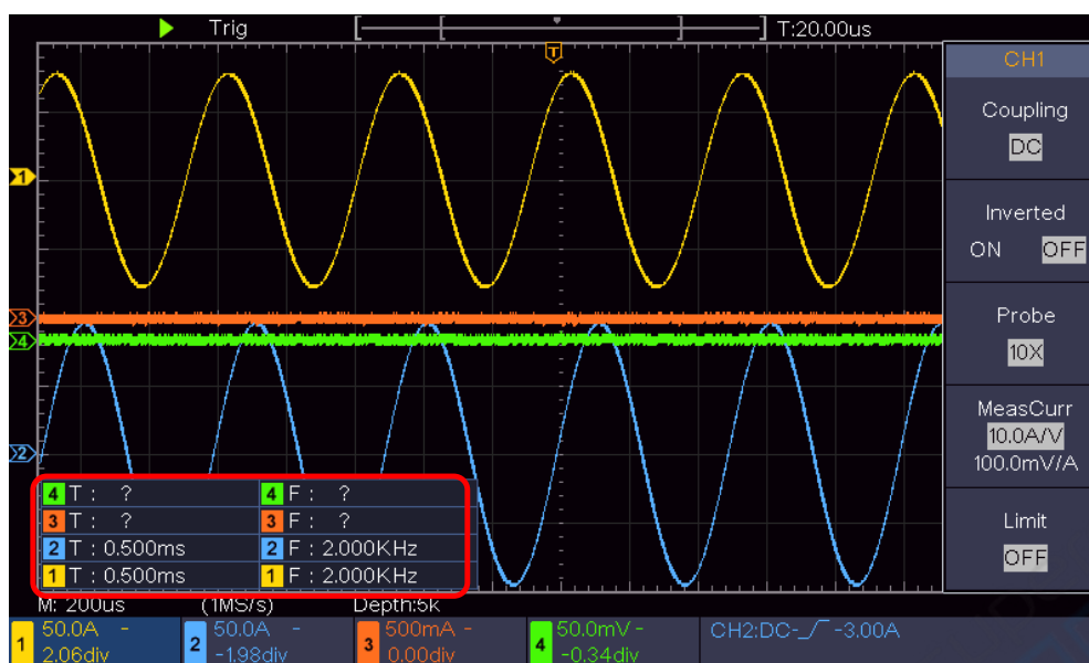
Figure 4-12 Automatic measurement
