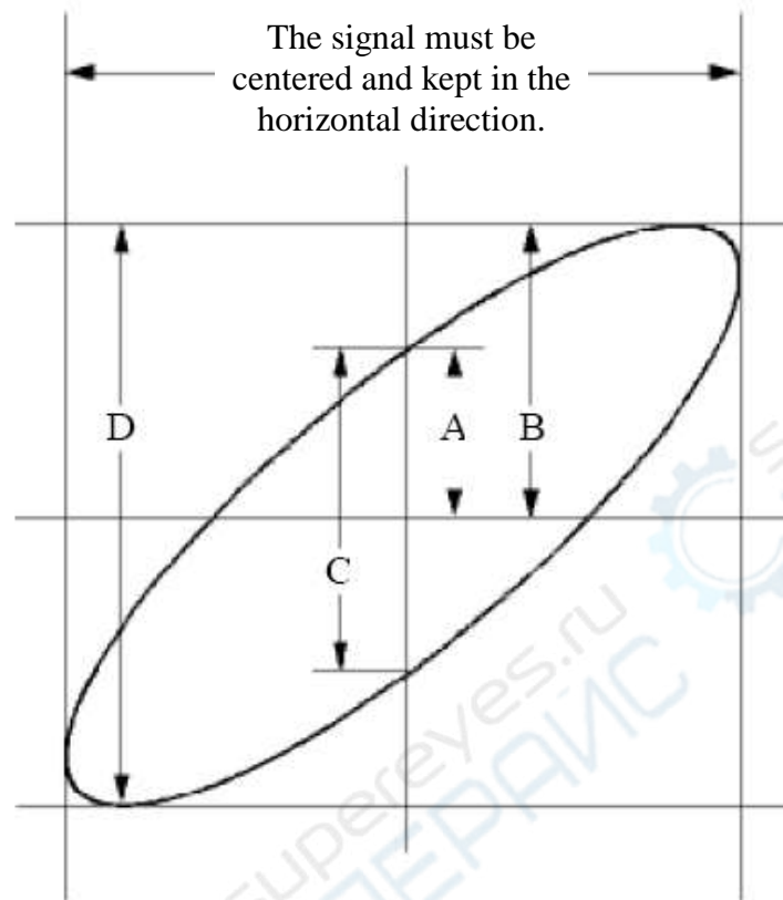
Figure 6-6 Lissajous Graph
