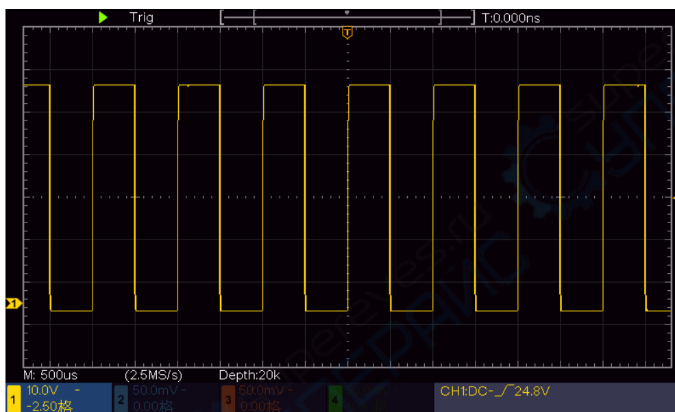
Figure 3-5 Auto set
