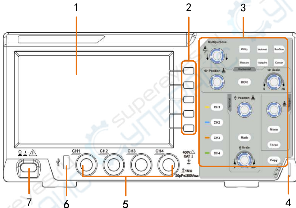
Figure 3-1 Front panel
