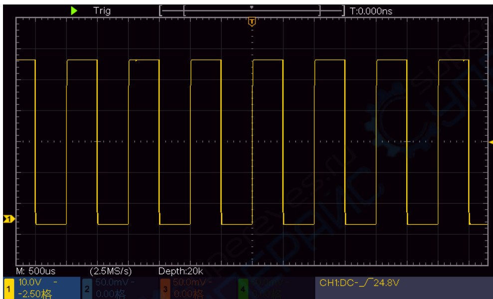
Figure 3-5 Auto set
