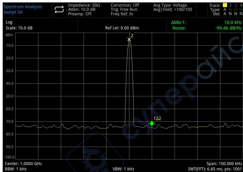
Figure 3-20 Phase Noise
