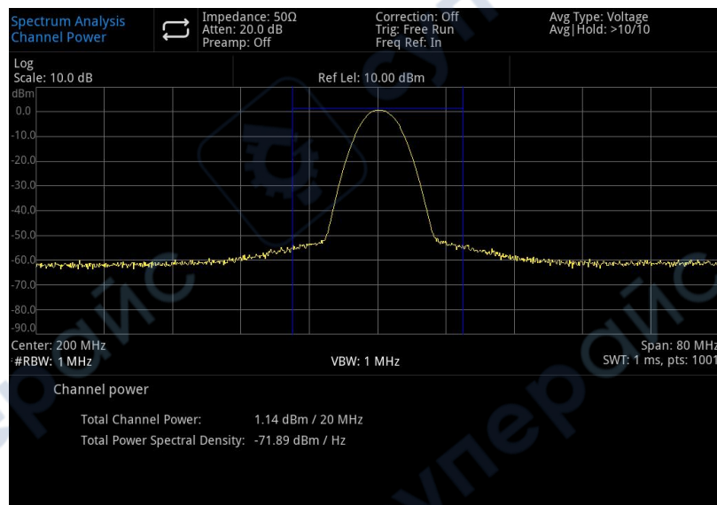
Figure 5-1 Channel Power
