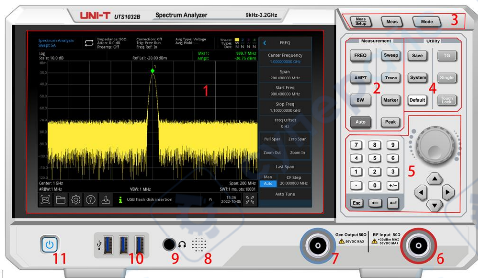
Figure 1-1 Front Panel
