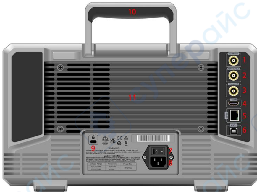
Figure 1-3 Rear Panel
