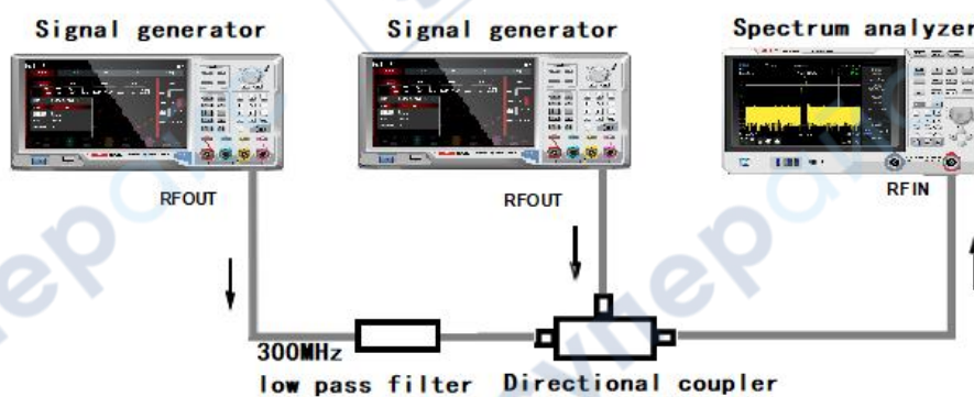
Figure 3-18 Instrument Setting of Third-Order Intercept Signal
