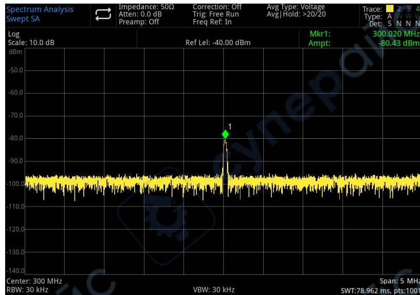
Figure 3-14 Trace Averaging
