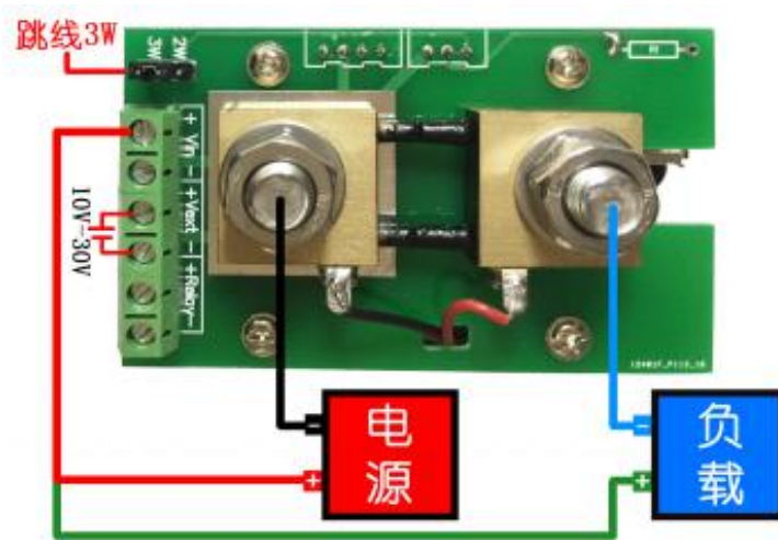
Figure 2-4Three-wire relay wiring diagram is not connected
