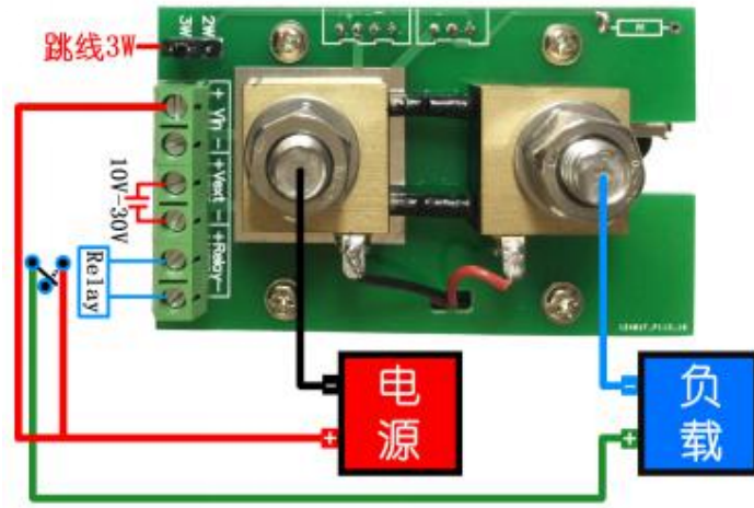
Figure 2-5 Three-wire connection Relay wiring diagram
