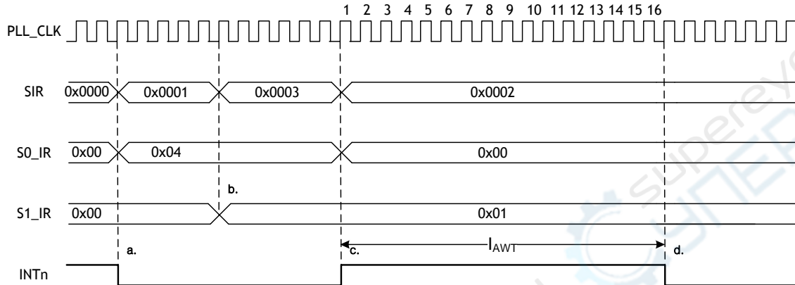
Figure 21. INTLEVEL Timing
