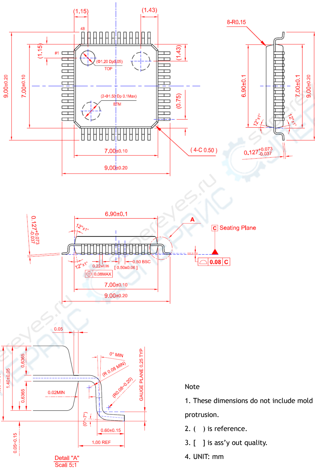
Figure 25. Package Dimensions
