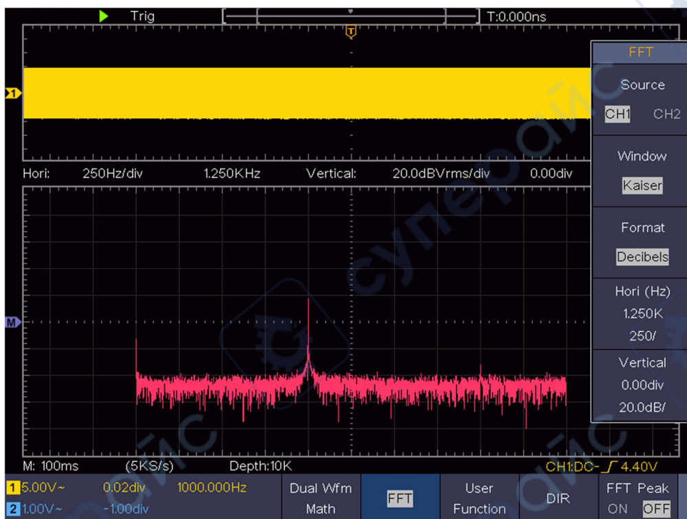
Figure 4- 5 Kaiser window
