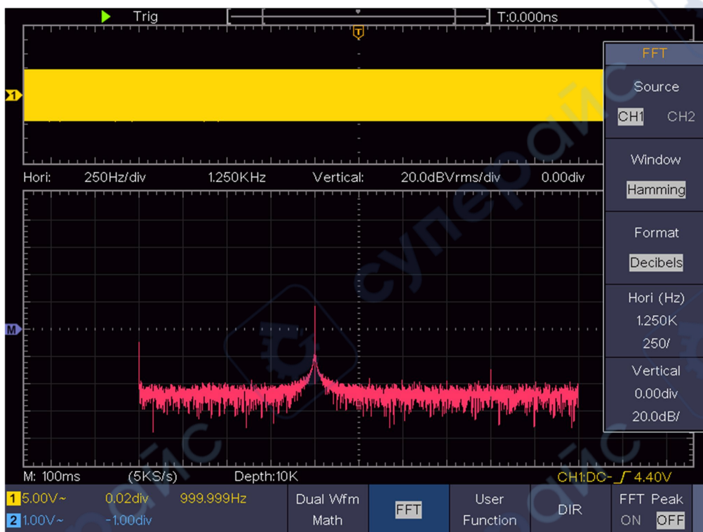
Figure 4- 1 Hamming window
