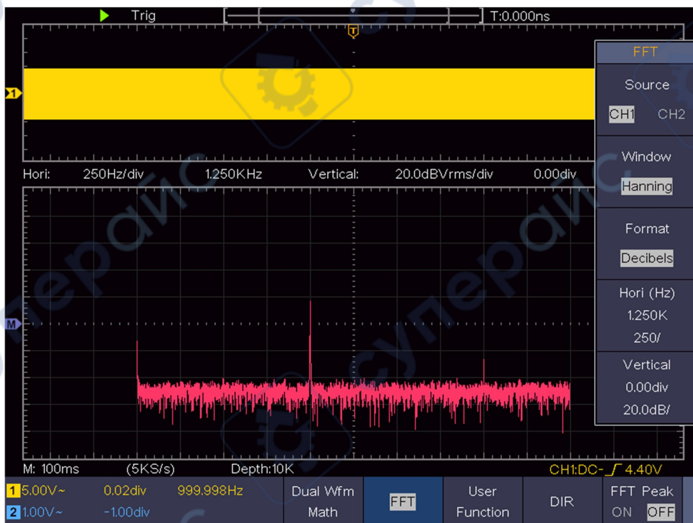
Figure 4-4 Hanning window
