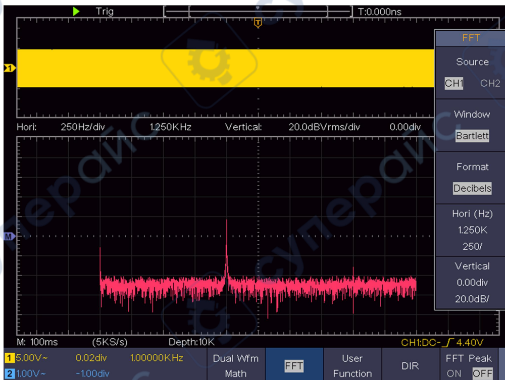
Figure 4- 6 Bartlett window
