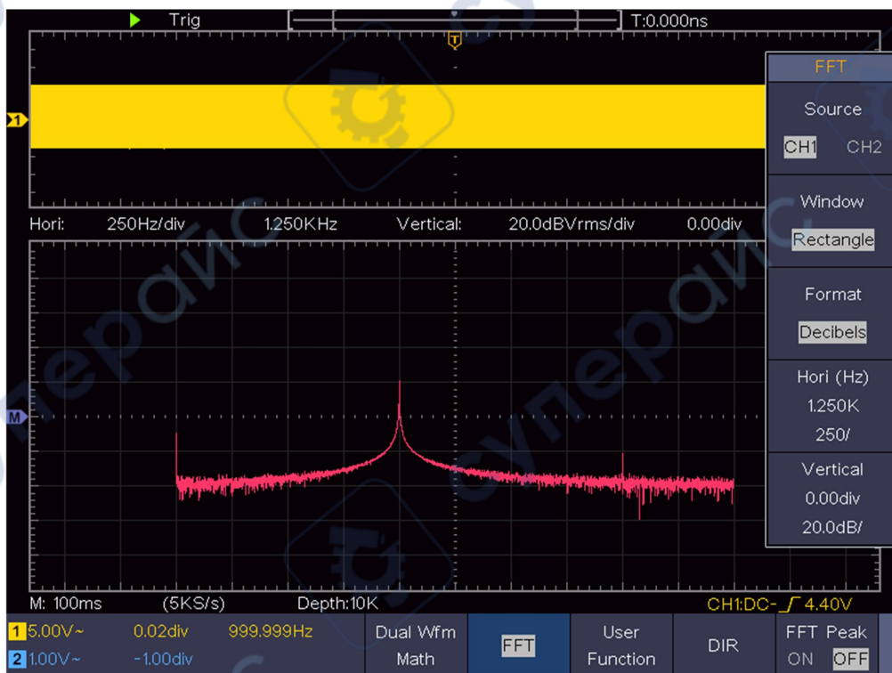
Figure 4- 2 Rectangle window
