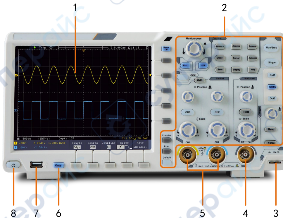
Figure 3- 1 Front panel
