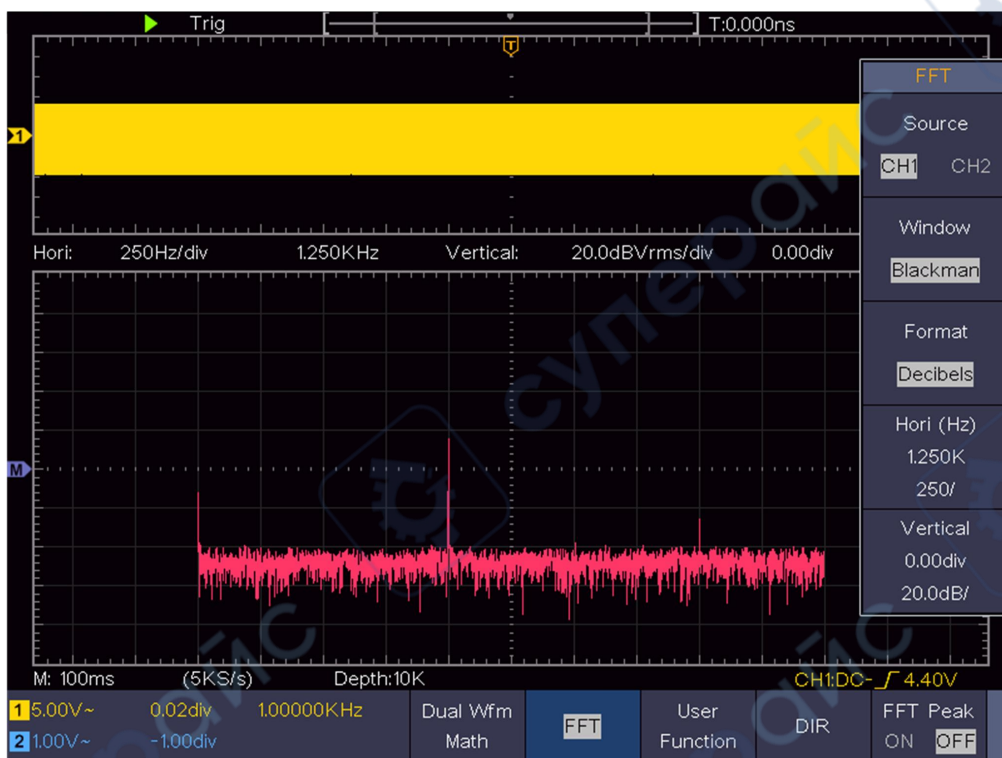
Figure 4-3 Blackman window
