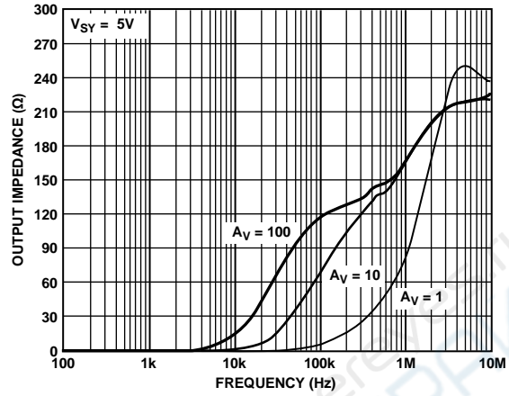
Figure 22. Output Impedance vs. Frequency at 5 V
