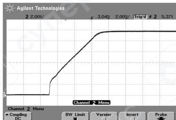
Enable Start-up (Vin=48V I OUT =30A)
