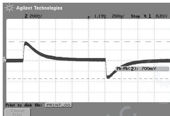
Transient Response (Load 50% to 75%)
