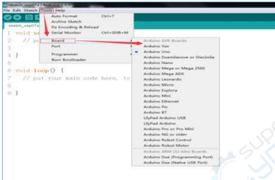
Figure 2.1.14 Tools interface
