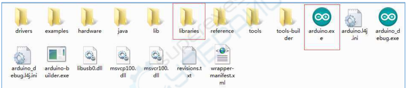
Figure 2.1.11 Software Catalog
