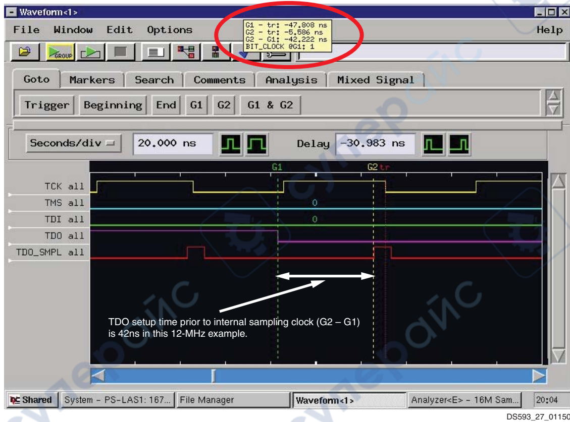
Figure 27: TDO Sampling Example at 12 MHz (TDO Setup Time Relative to Sampling Point)
