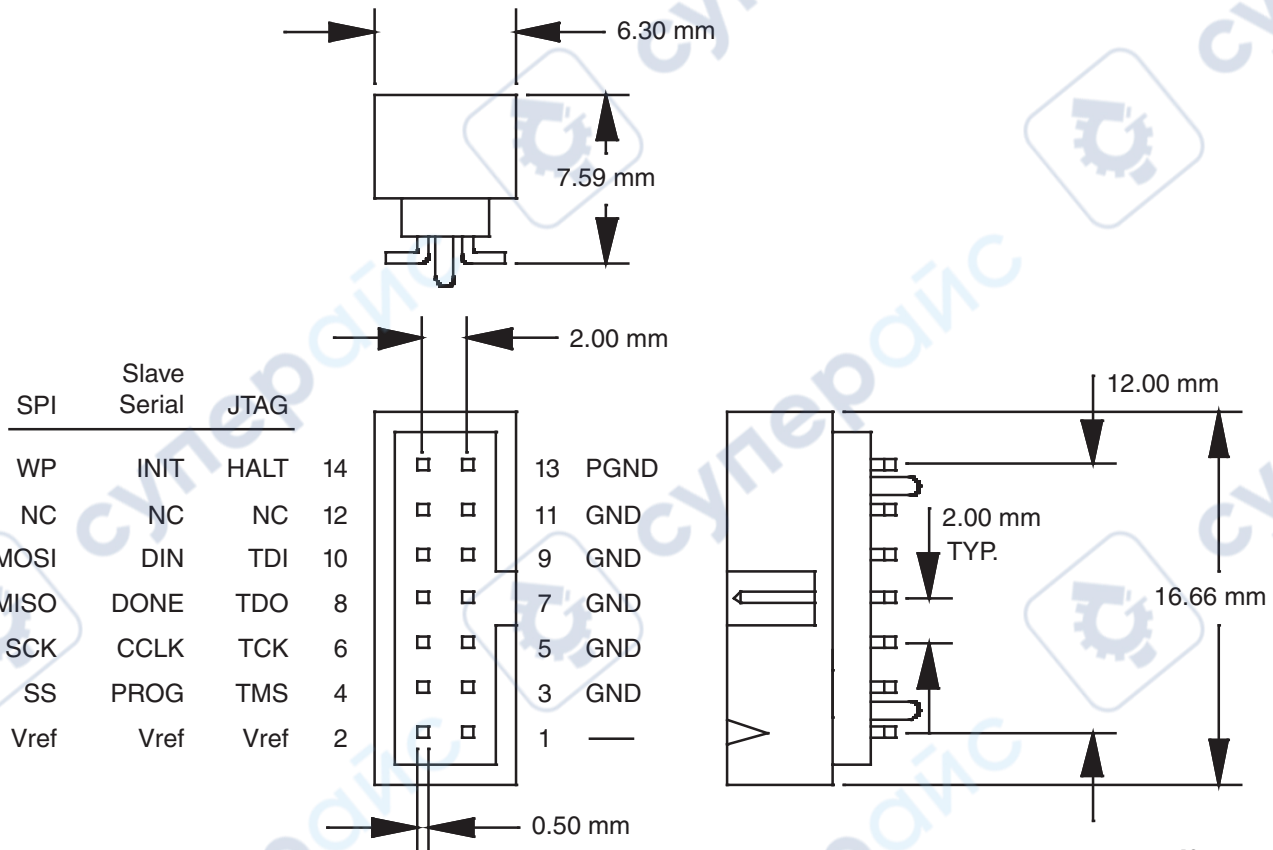
Figure 14: Target Interface Connector Dimensions and Signal Assignments
