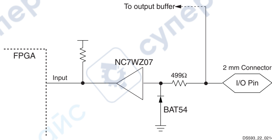
Figure 22: Target Interface Receiver Topology
