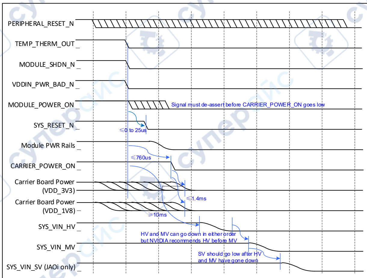
Figure 5-5. Power Down Sequence – Shutdown Due to an Event Case
