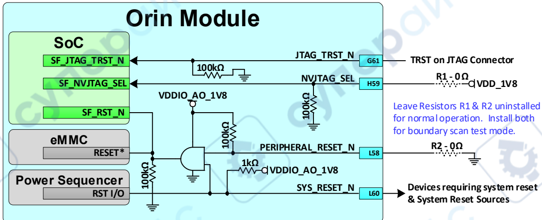
Figure 20-1. Boundary Scan Connections
