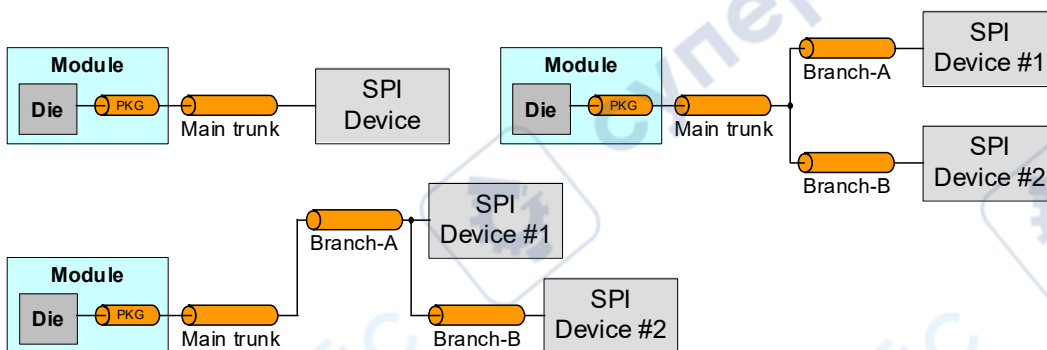
Figure 14-3. SPI Topologies
