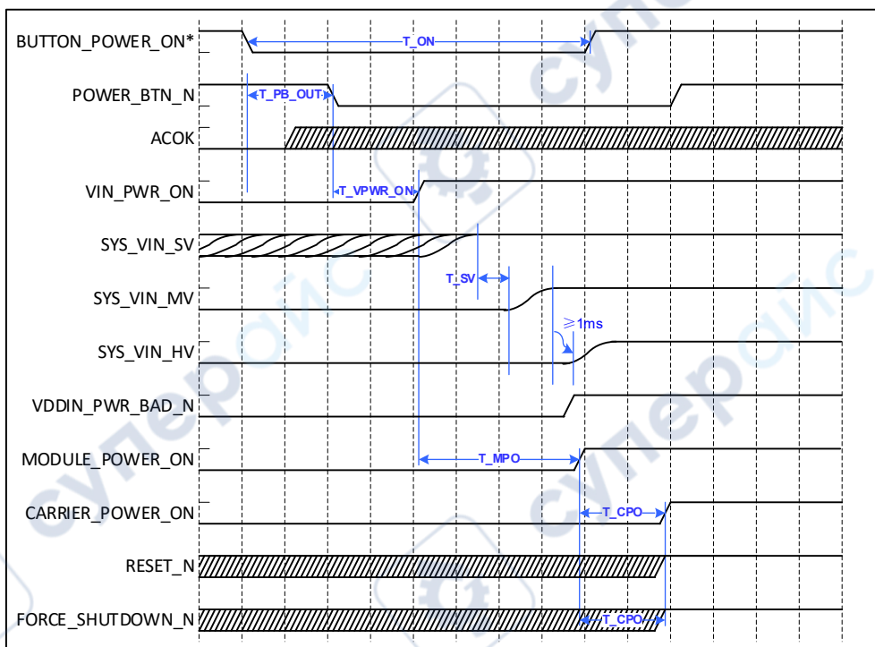
Figure 5-8. Power-OFF to On Sequence Power Button Case
