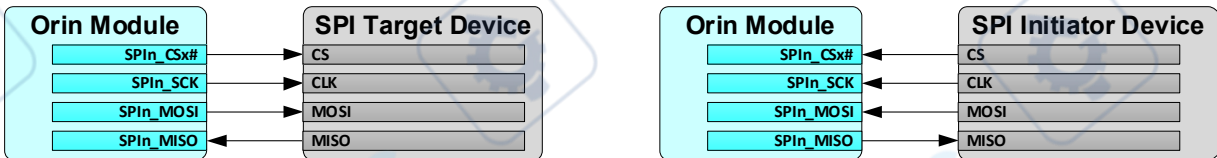
Figure 14-2. Basic SPI Connections
