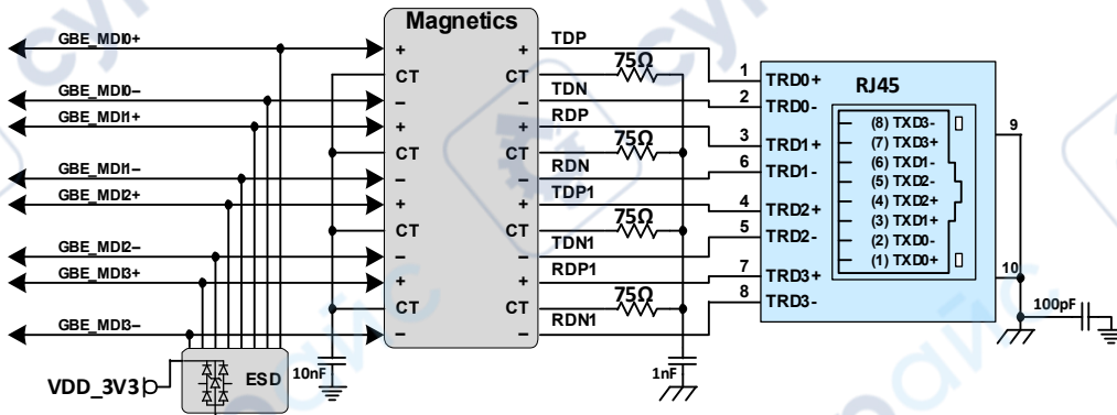
Figure 8-2. Gigabit Ethernet Magnetics and RJ45 Connections
