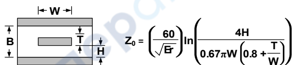
Figure 26-3. Stripline Transmission Line
