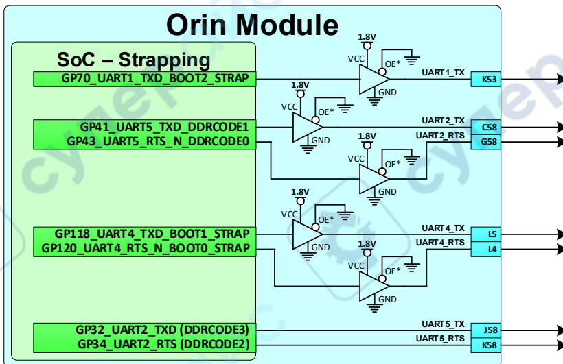
Figure 19-2. Orin Module Strap Pins
