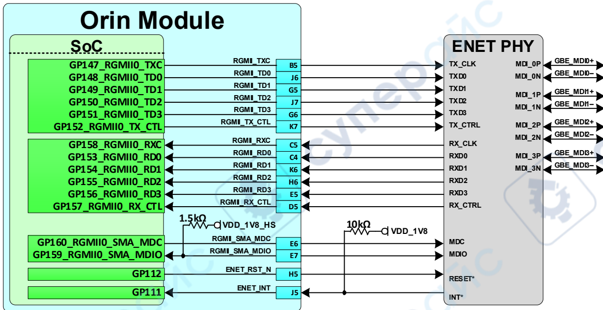
Figure 8-1. Ethernet Connections
