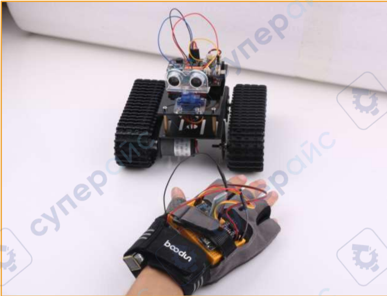
Figure 31: Gesture Control Panther-tank
