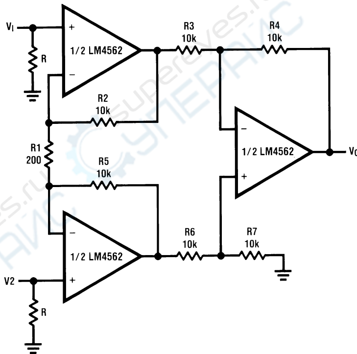
Figure 126. RIAA Preamp
