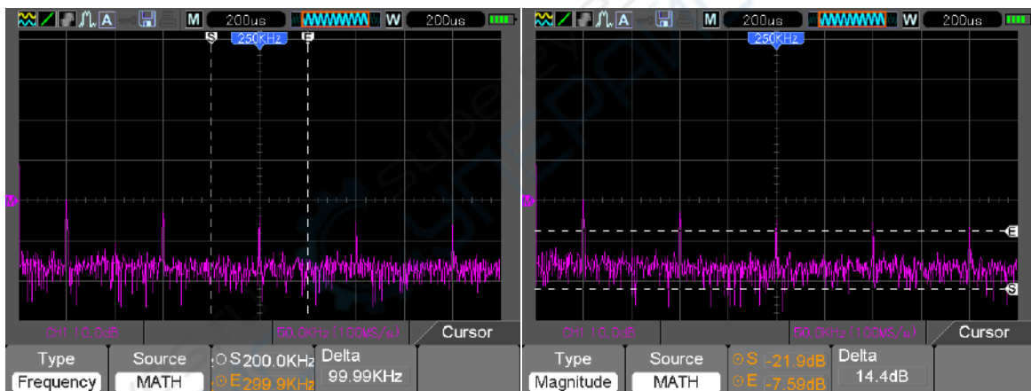
Frequency Cursors
