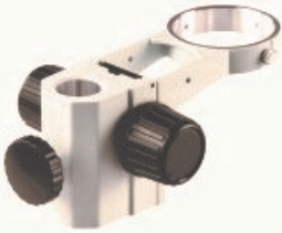
A1 Focusing Mount ID.32mm for Pole ID.76mm for Microscope Body Dist. Centre-to-centre:155mm The Vertical W.D.:50mm
