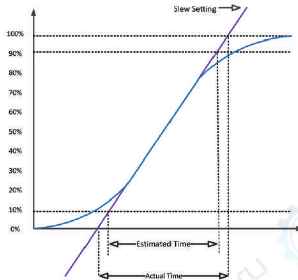
▲ Slew Rate and Actual Transition Time
