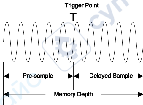
Figure 4-3 Memory Depth
