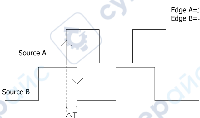
Figure 5-10 Delay Trigger
