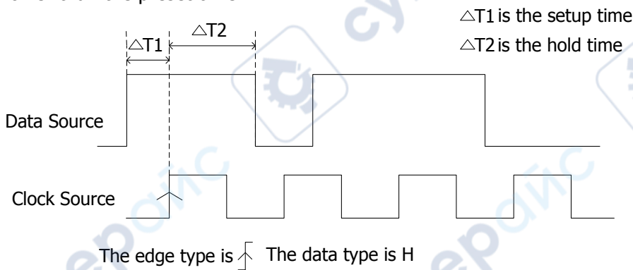
Figure 5-11 Setup/Hold Trigger
