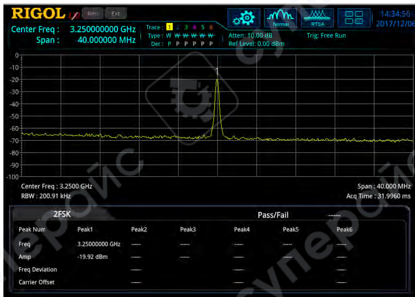
Figure 3-8 SSC Measurement Interface
