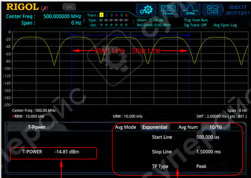
Measurement Result Measurement Parameters Figure 2-5 T-Power Measurement Interface
